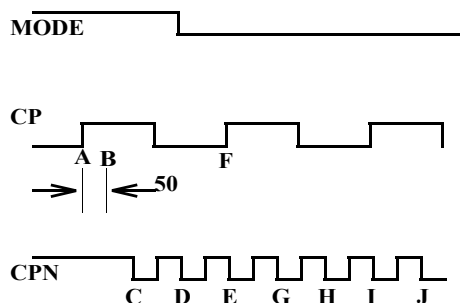
Figure 31-1—Sample $timeskew
